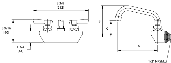
Dimensions shown in inches (mm) are for reference only and are subject to change.
